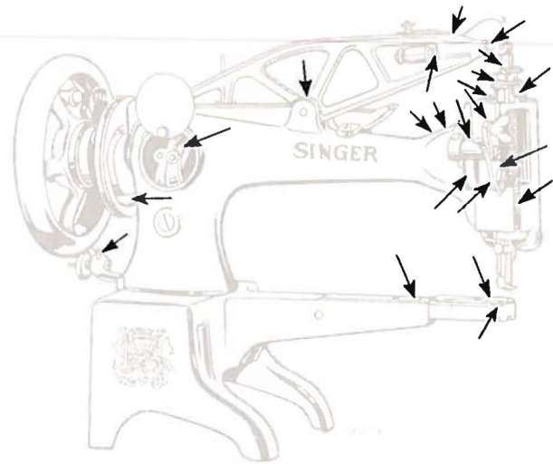
Fig. 3. Oiling Rear of Machine
