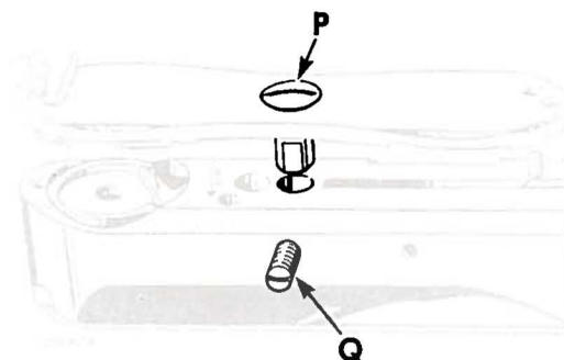
Fig. 33. Correct Position of Hinge Pin in Needle Plate
