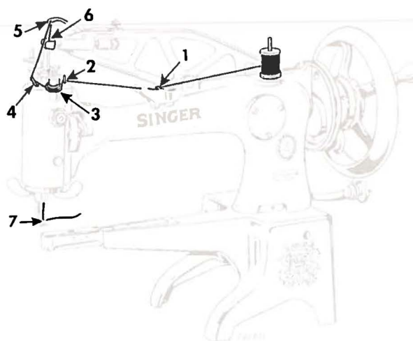
Fig. 19. Threading Needle
